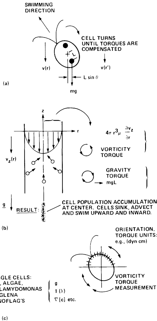
Fig. 1. (a) Orientation of cell is determined by torque compensation: mgL \sin is the gravity torque (clockwise). The vorticity torque is also clockwise, since v(r') > v(r) . This situation prevails in (b), left-hand side of diagram. For torque compensation, the cell turns until it is oriented as in (b), left-hand side. (c) illustrates possible replacements for the gravity torque, illumination I(\lambda) and chemical concentration gradient \nabla[c] .
